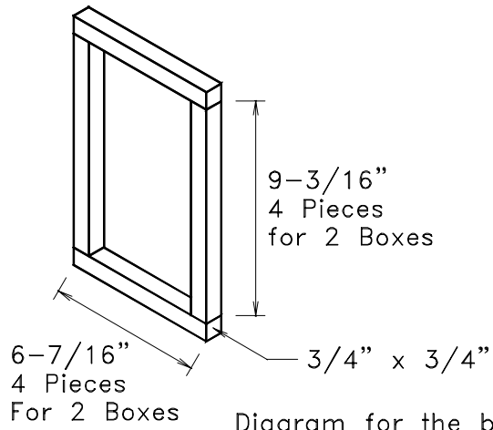
Diagram for the bracing around the back openings of the satellites.
